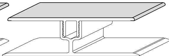
união clip alum. 60mm * alum. jointer clip 60mm * liaison à clipser alum. 60mm *
